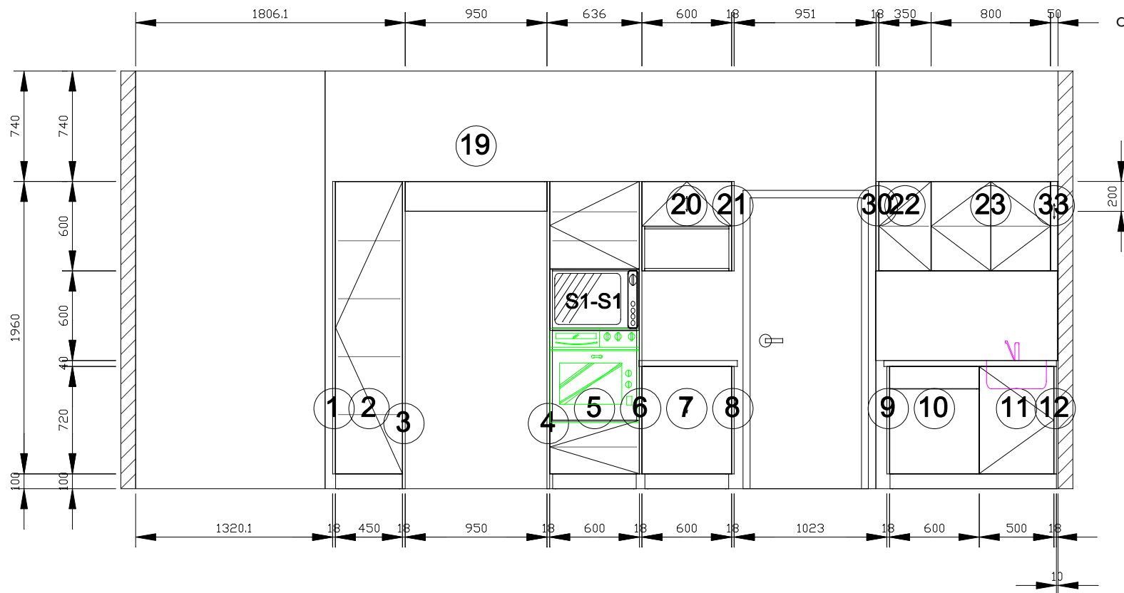
A View elevation drawing
